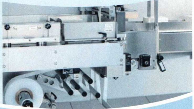
Film unwind with cross pushing function and sealing station
