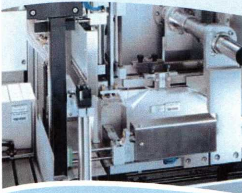
Cross sealing station and folding function
