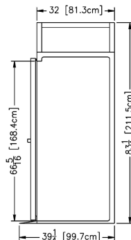
Section - RET232LUT-FHS
