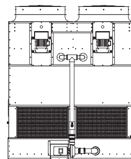
Pump Elevation
