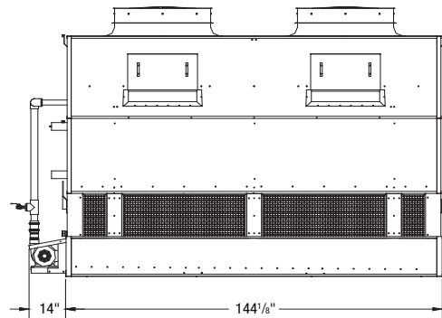
Side Elevation MW44-MW44C
