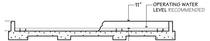
Section-Flat Slab Basin
