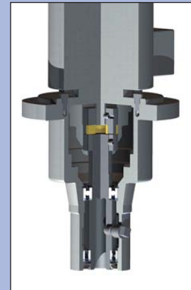
Direct Drive Section View
