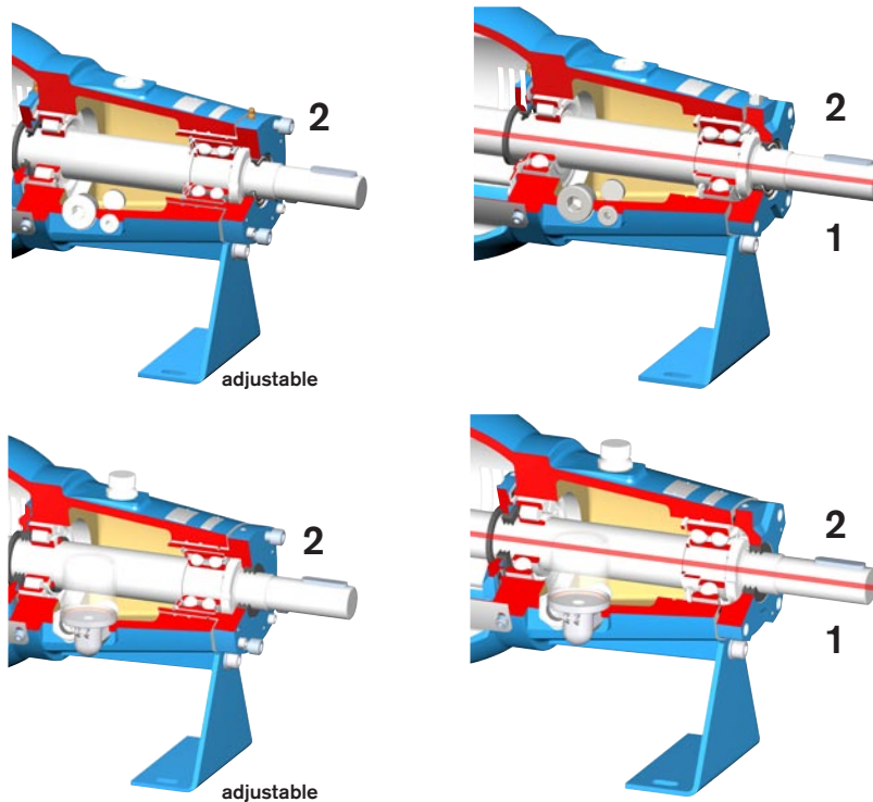
Grease lubrication
