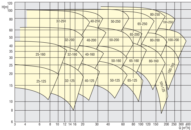
n_{nom} = 3000 \text{ rpm} (Motor 2 polos - 50 Hz)
