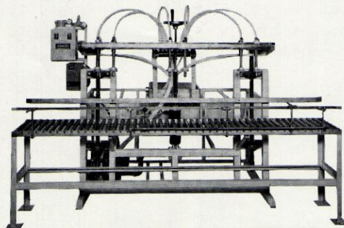
Model "400" Pressure Filler
