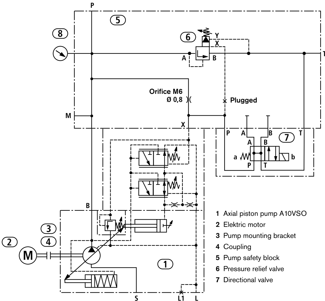
Axial piston pump with pressure, flow and power controller with pressure safety and start-up assistance
