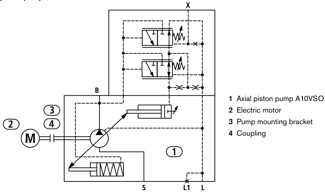
Axial piston pump (basic version)
