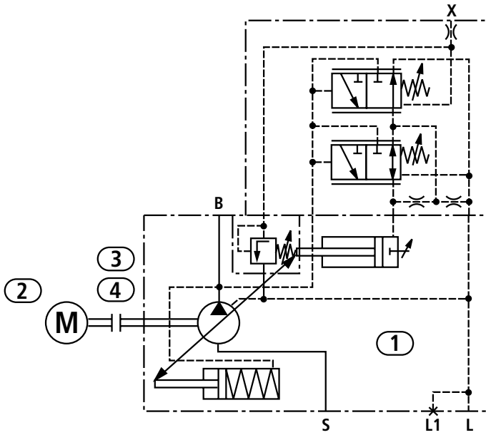
Axial piston pump with pressure, flow and power controller (basic version)
