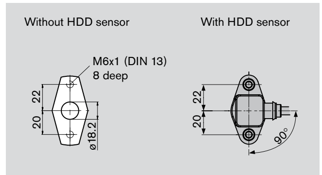
View X
