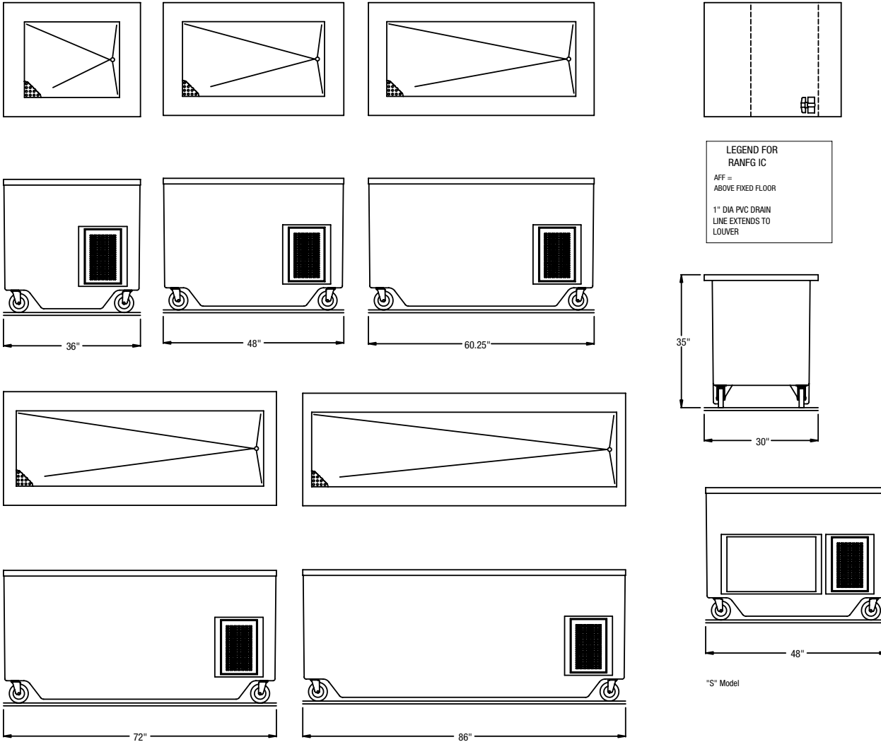
RANFG-IC DRAWINGS SHOWN, RANFG IC-S FRONT VIEW SHOWN AS REPRESENTATION OF "S" MODELS Drawings are to be viewed in the same order as the chart
