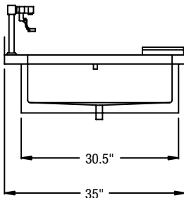
CONDIMENT PAN HOLDING ASSEMBLY SUPPLIED W/(8) 1/9 SIZE PANS, EACH PAN 2 1/2" DEEP
