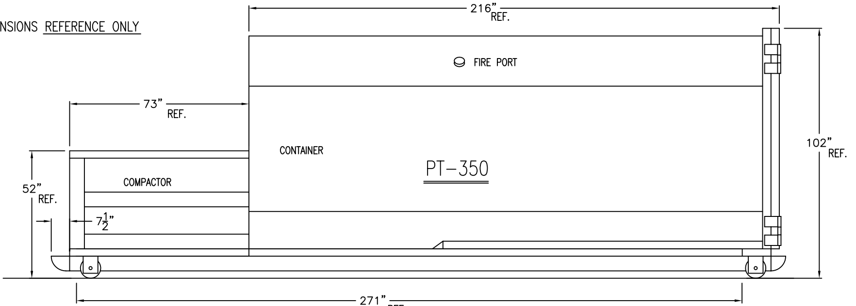
SIDE VIEW
