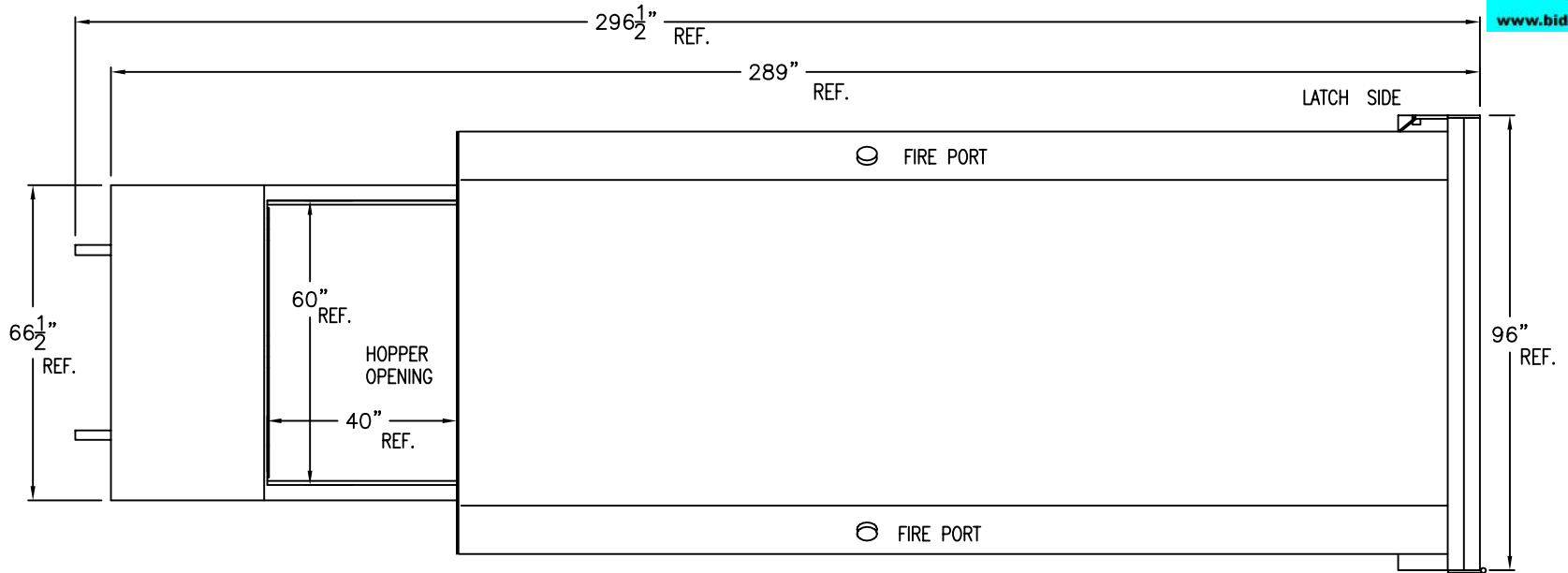
TOP VIEW
