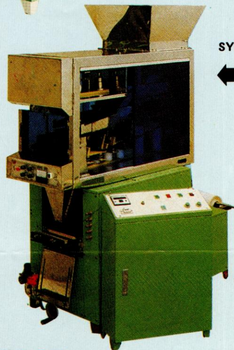
自動計量器 SY-20W Automatic Weighing Device 400 x 1100 x 900 mm Power: 250W Capacity: Model A 50g-1kg Model B 250g-3kg
