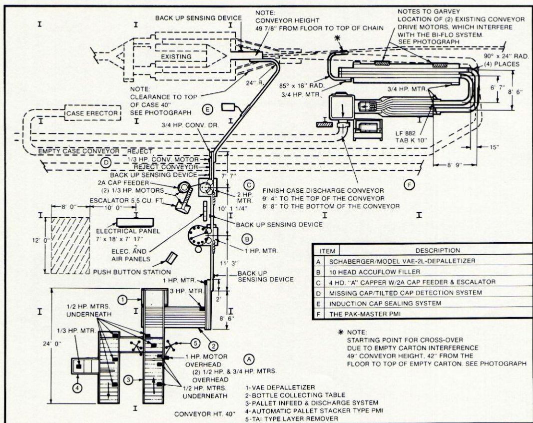
Typical Turnkey Layout
