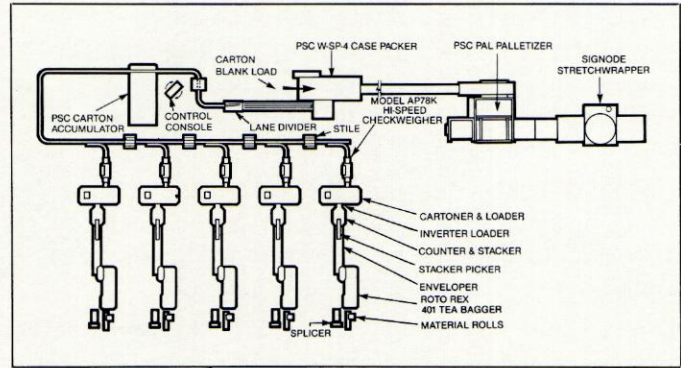
Typical Turnkey Layout
