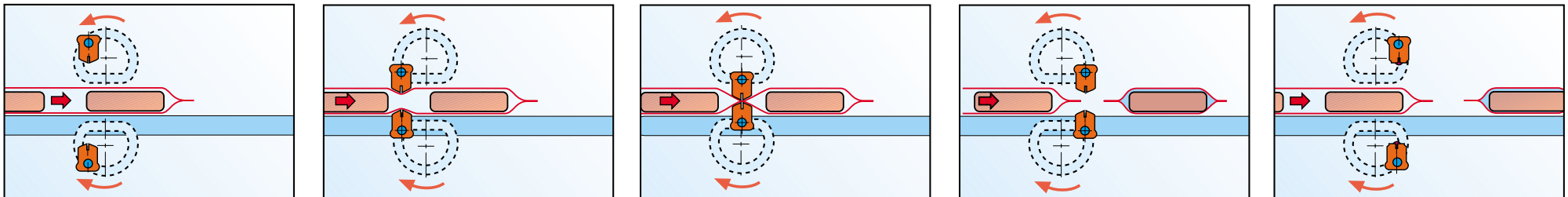
The Long Dwell sealing system (patented PFM): one jaw per jaw support, superior flexibility, up to 140 cycles/min.
