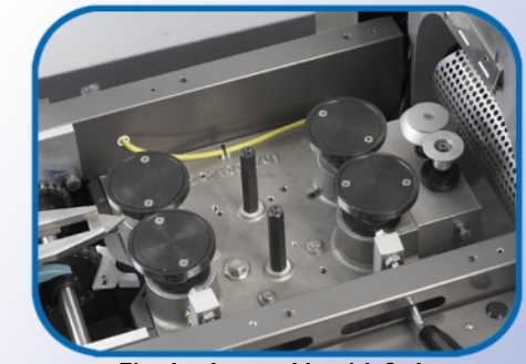
Finwheel assembly with 3rd set of foldover wheels
