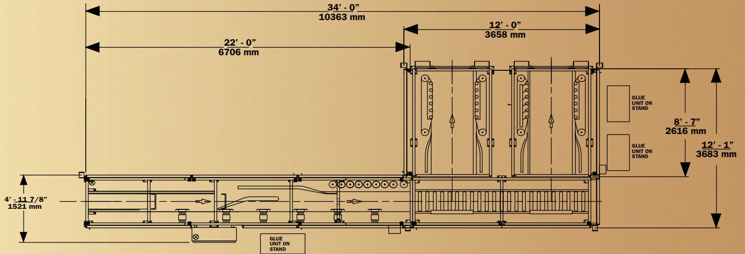
PLAN VIEW
