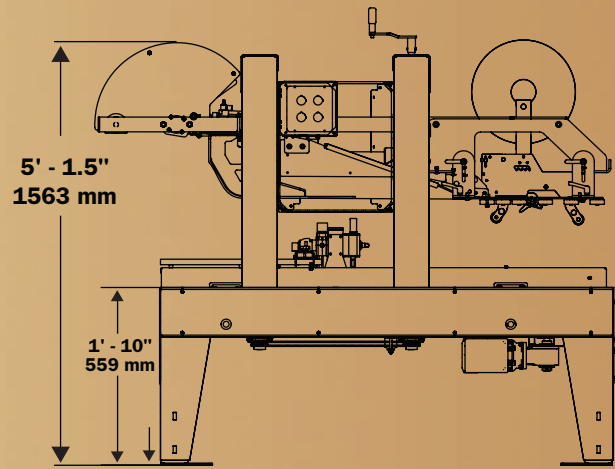
ELEVATION VIEW
