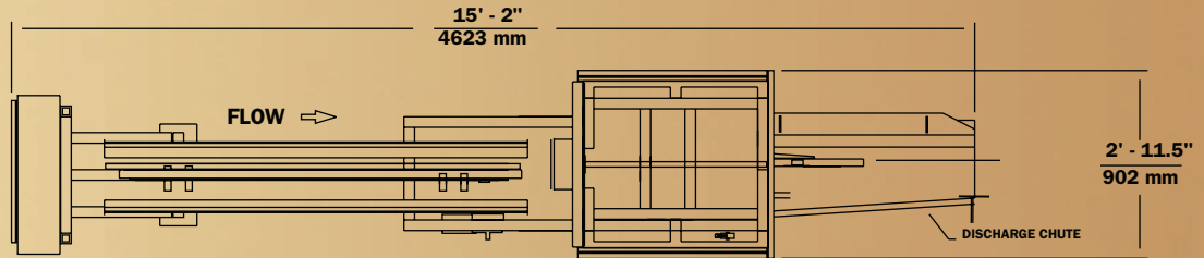
Plan View
