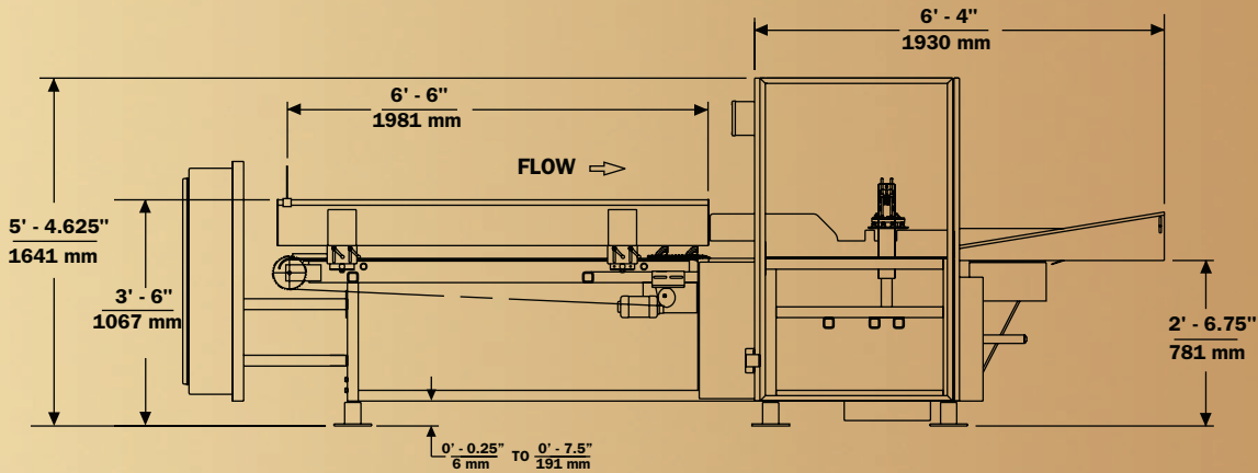
Elevation View
