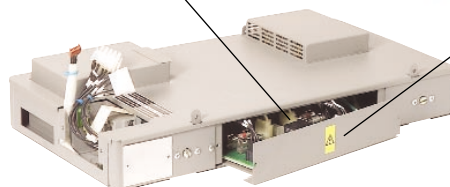
Works-in-a-drawer design makes fuses easily accessible from front of melter
