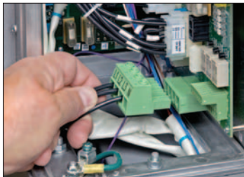
Quick disconnect plug for easy input voltage connection
