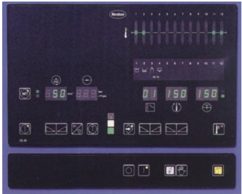
Standardized international symbols on the CS 20 operator panel and gas panel provide easy understanding and safe operation.
