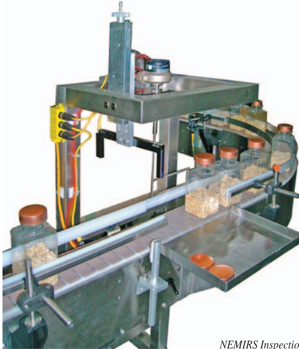
NEMIRS Inspection/Rejection System (Shown without guarding)
