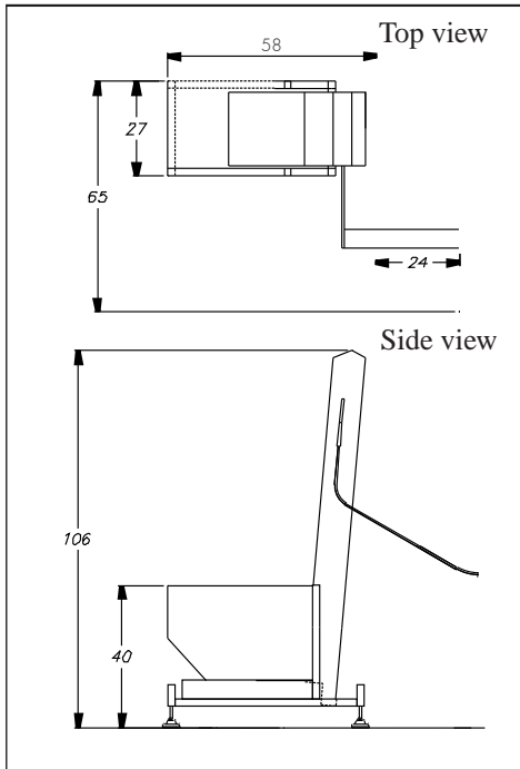
Single line cap sorter elevator
