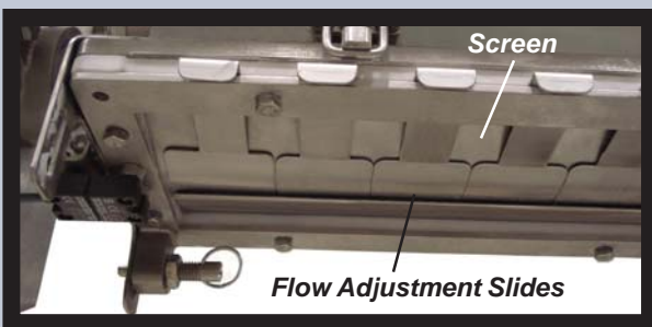
Flow Adjustment Assembly Components (viewed from below)
