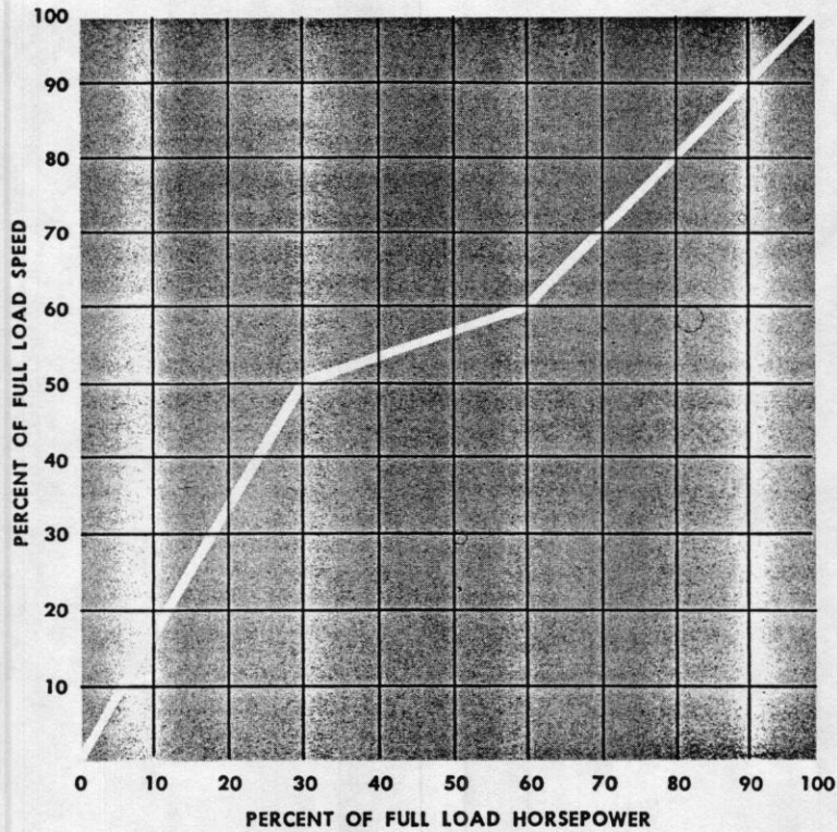
Typical rating curve for Vari-Mix units
