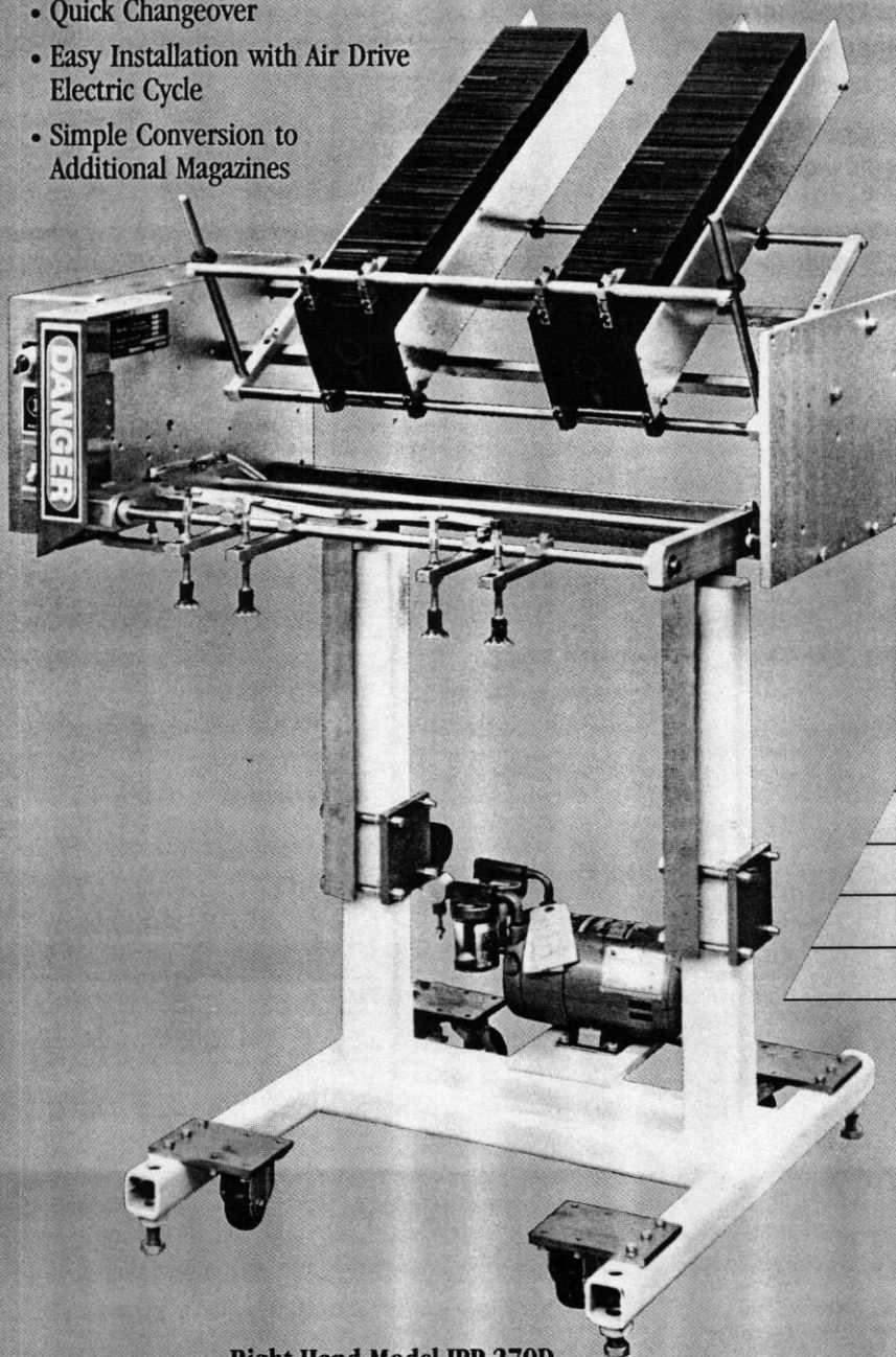
Right Hand Model IPP-270D (28" Wide) with 30" Magazines, Floor Stand with Casters and Vacuum Pump
