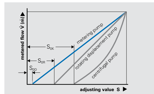
Advantage of the metering pump: the pressure stiff characteristics
