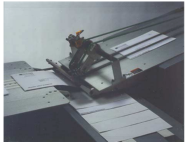
An in-line divert gate removes mixed mail, purged or non-printed mail pieces from the system
