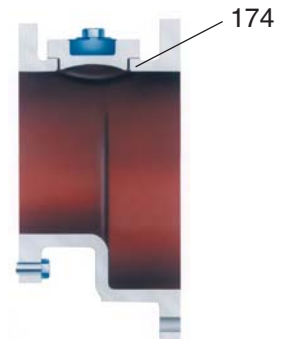
Optional Suction Piece
