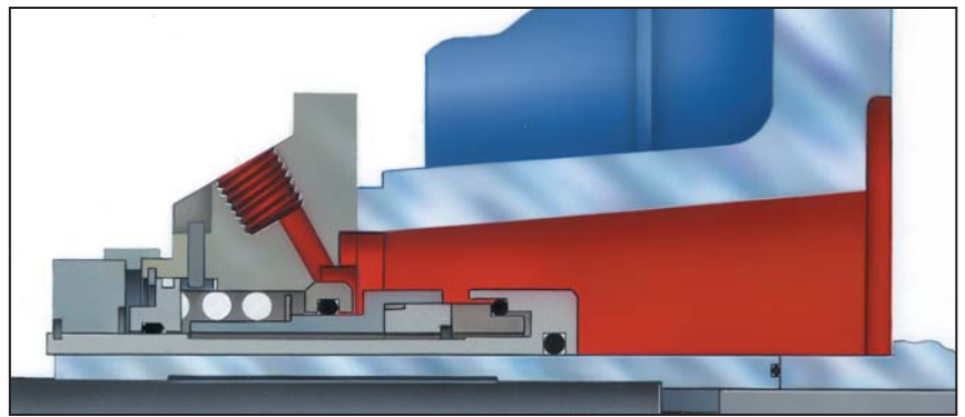
TaperBore™ Seal Chamber and Mechanical Seal Option
