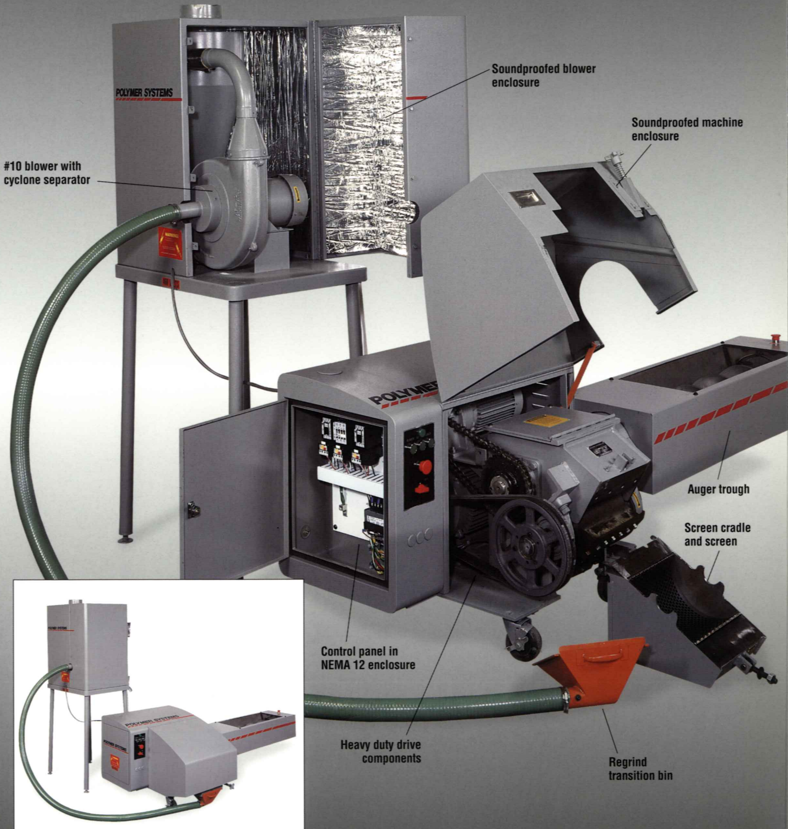
Model 1010A with soundproofed blower evacuation system.
