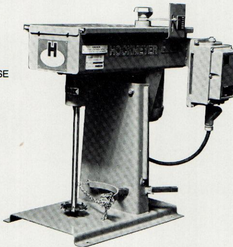
2 HORSEPOWER, MODEL 2L, LAB MODEL
