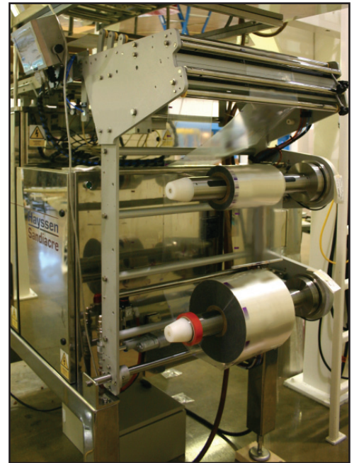
Reduce setup times with film splicing, film reel runout device and easy thread film path
