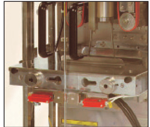
Servo-driven, intermittent motion cross seal jaws.
