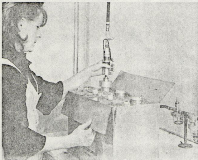
Capping two gallon cans in the case with an HCH-18 portable hand capper.
