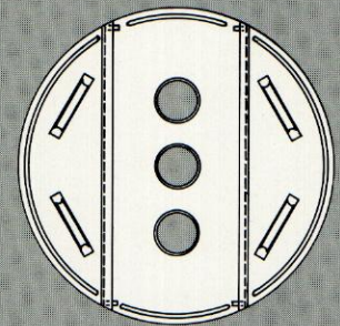
Style #8 Three piece hinged lift-off type 150 to 500 gallon size triple action mix cooker
