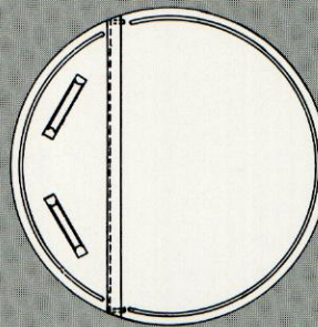
Style #3a Two piece hinged lift-off type 15 to 500 gallon size for open top kettle
