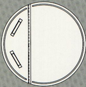
Style #2a Two piece lift-off type 15 to 500 gallon size for open top kettle
