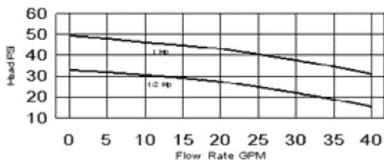
Pump Performance
