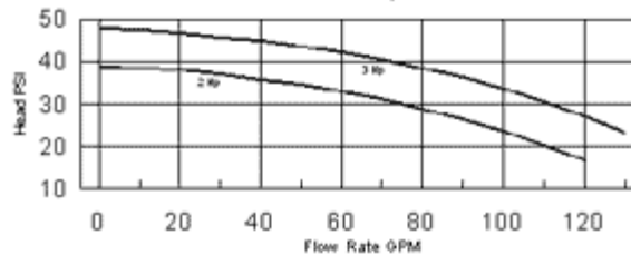
Pump Performance
