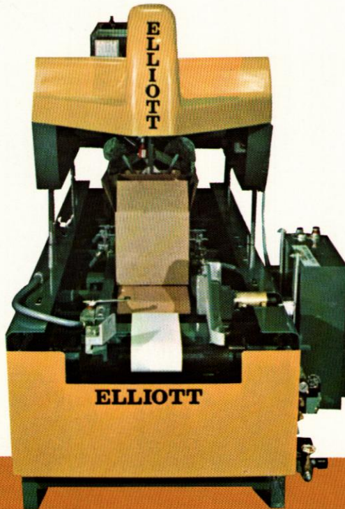
Feed End View of HMT-Mini Model
