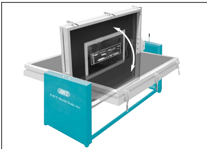
Counterbalanced design allows smooth and effortless rotation of the Photo Select Clear plate glass top from a horizontal position for use with overhead or underside lighting, to a vertical position for front exposing systems.
