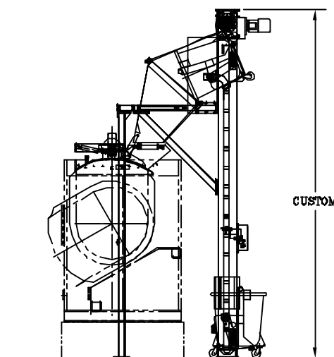
TROUGH HOIST-MIXER
