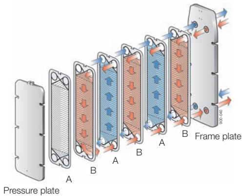
Flow principle of a plate heat exchanger
