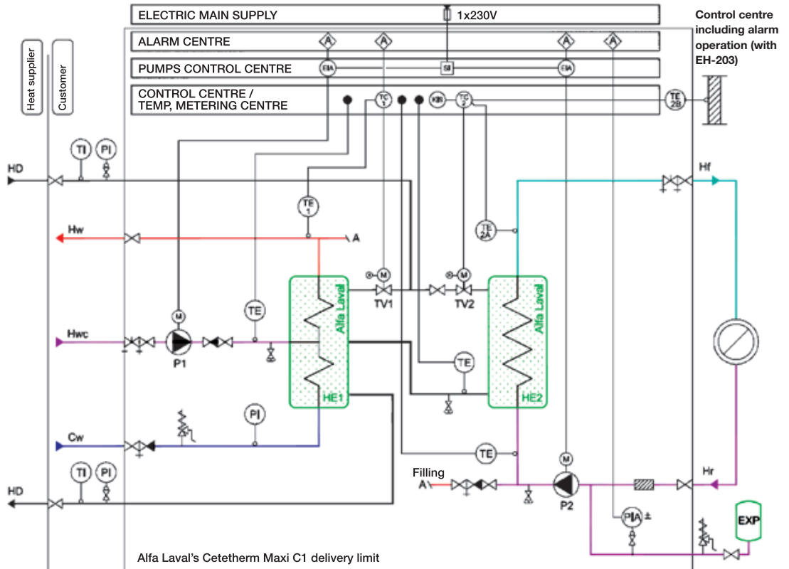
Typical flow chart for Cetetherm Maxi C1. Components can vary due to individual calculations.
